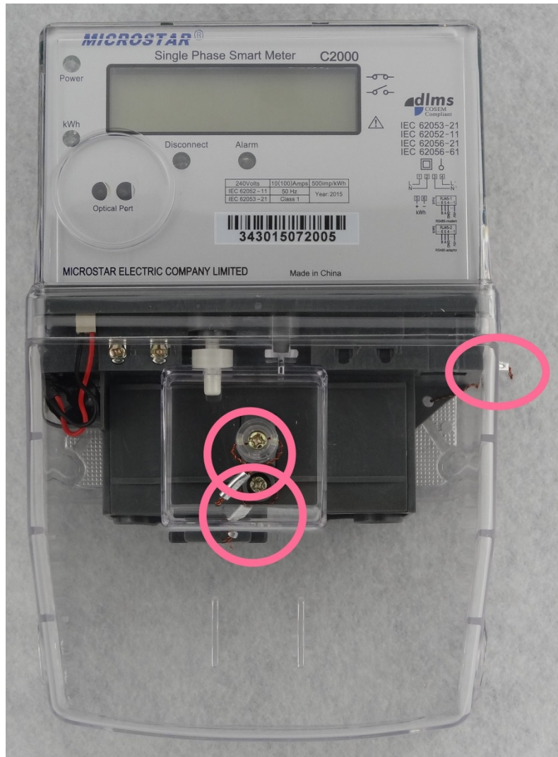
Microstar Model C2000 (Including Typical Mechanical Sealing)
